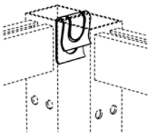
Connection clamp, Model VBKL For connecting the bearing frames of two adjacent shelving sections, very helpful for extremely high bays or for precise adjustment of the bearing frames, one each is required per shelf connection. Bright galvanized metal.
