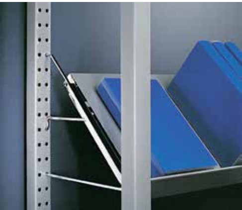
Slanting brace, Model SSTB For variable slanting of shelves with book stop (edge), for display and front presentation; two each slanting braces required per shelf; round steel, bright galvanized.
