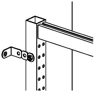
Wall fastening, Model WBEF For single-sided bays with more than 1100 mm height; bright galvanized metal, incl. fastening kit. Wall distance 0 – 40 mm.
