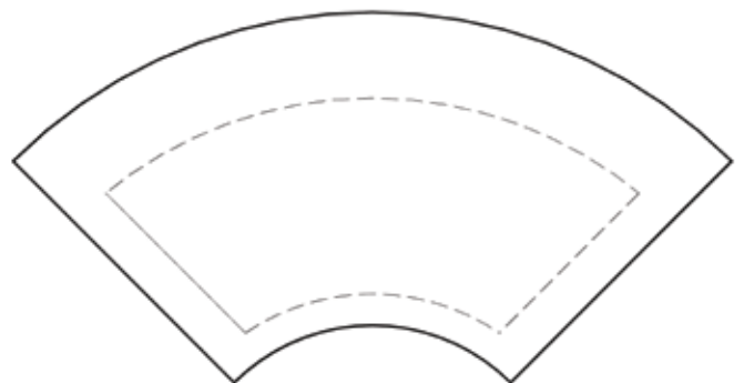
RFID installation in 90° curved counters
